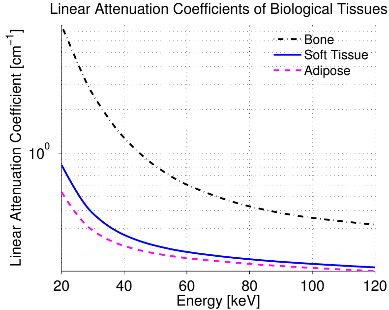
Figure 2.3: Linear attenuation coefficient values for biological tissues in the diagnostic energy range [27].
