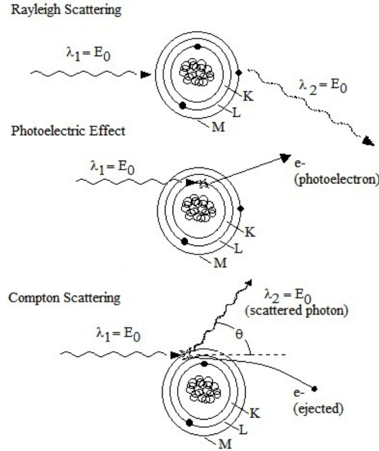
Figure 2.2: X-ray interactions with matter. E_0 is the energy of the incident photon, \lambda_1 . \lambda_2 is the scattered photon, and e^- is an electron.
