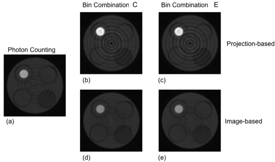
Figure 5.3: Reconstructed energy-weighted image. Shown are images reconstructed using (a) photon-counting; (b) projection-based weighting with bin combination C; (c) projection-based weighting with bin combination E; (d) image-based weighting with bin combination C; (e) image-based weighting with bin combination E. All images have the same window (6000 HU) and level (1800 HU).
