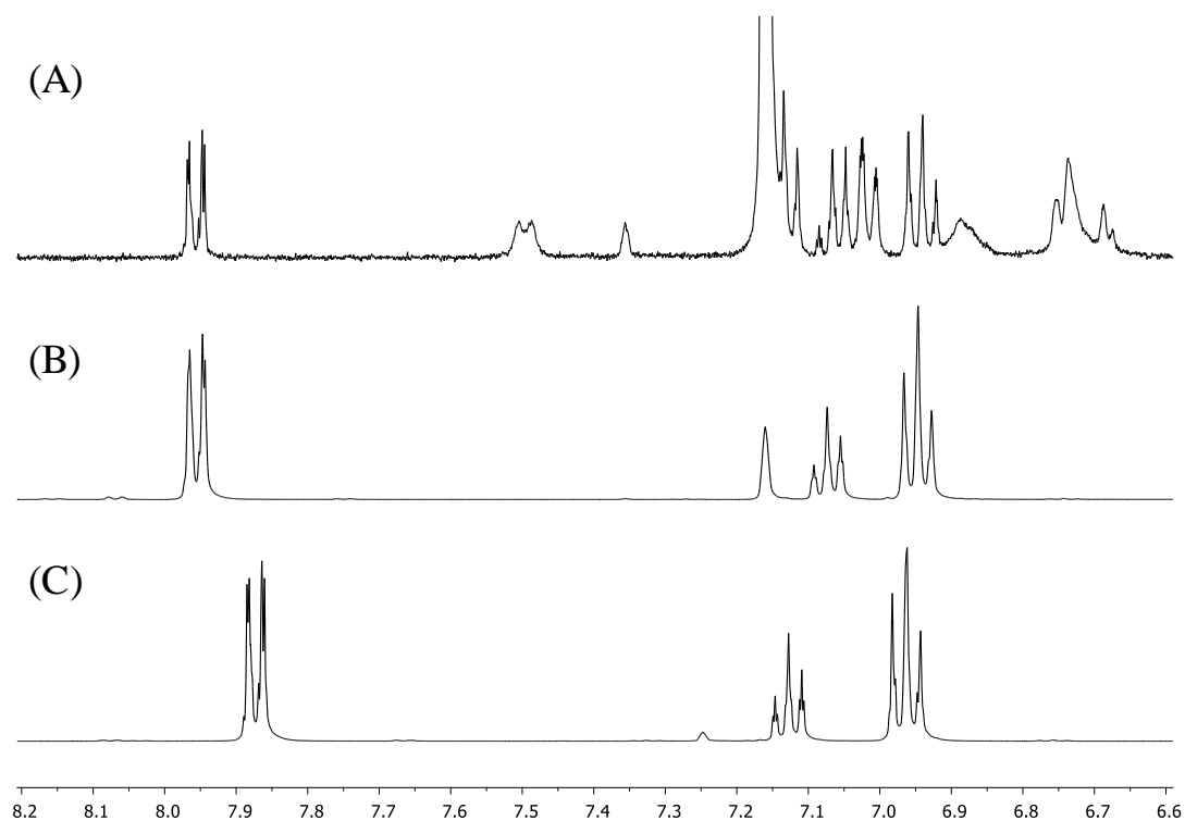
Figure S16. Comparison of ^1\text{H} NMR (400 MHz, \text{C}_6\text{D}_6 ) of reaction products from 2 + \text{N}_2\text{O} using benzoyl chloride as an oxygen trap to form benzoic anhydride (A); authentic sample of benzoic anhydride (B); authentic sample of benzoyl chloride (C).
