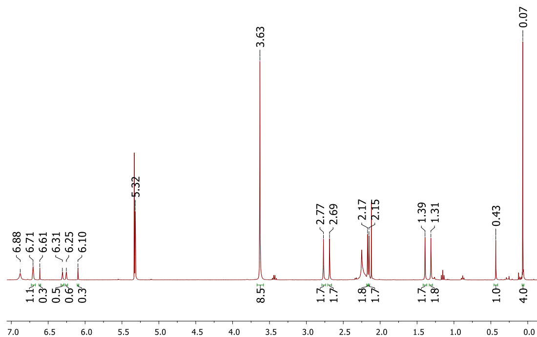
Figure S13. ^1\text{H} NMR (400 MHz, \text{CD}_2\text{Cl}_2 ) of reaction products from 2 + \text{N}_2\text{O} , using 5 equivalents of TMS-Cl as an oxygen trap. Hexamethyldisiloxane appearing at 0.07 ppm is the major product and some unreacted TMS-Cl appears at 0.43 ppm. Residual solvents in spectra are not peak picked.
