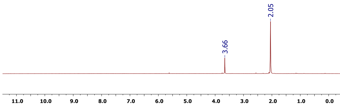
Figure S6. ^1\text{H} NMR (500 MHz) of 2 in Acetone- \text{d}_6 .
