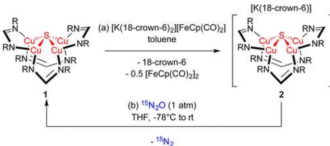
Scheme 1. Synthetic Cycle for N 2 O Reduction
