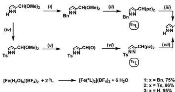
Scheme 1 Preparation of new scorpionates and iron(II) complexes. Key: (i) NaH, BnBr, THF; (ii) 2 Hpz, 5 mol% pTsOH·H 2 O, C 6 H 6 ; (iii) KO t Bu, dmsO, O 2 ; (iv) TsCl, NaOH, CH 2 Cl 2 ; (v) cat. CF 3 CO 2 H, H 2 O, EtOAc; (vi) S(O)pz 2 , cat. CoCl 2 , THF; (vii) NaOH (aq), THF, 5 min.
