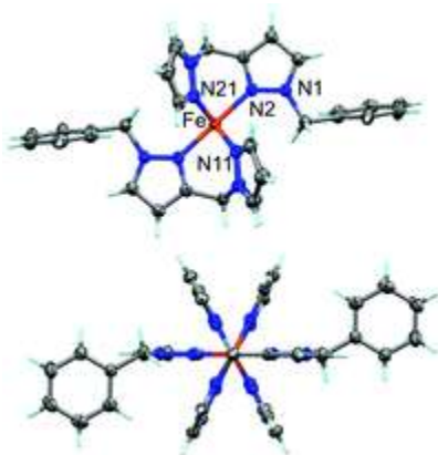
Fig. 3 Two views of the solid state structure of the dication in 1 ·2CH 3 CN. Thermal ellipsoids shown at 30% probability.
