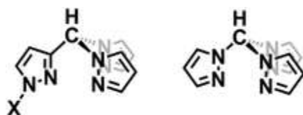
Fig. 1 Left: N-Confused tris(pyrazolyl)methane derivatives reported here ( \text{X} = \text{H} , \text{CH}_2\text{C}_6\text{H}_5 = \text{Bn} , \text{p-SO}_2\text{C}_6\text{H}_4\text{CH}_3 = \text{Ts} ). Right: Normal tris(pyrazolyl)methane.
