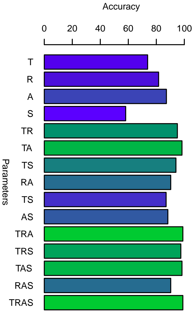
Figure 6.6: Accuracy for Man1 Varying Input Parameters
