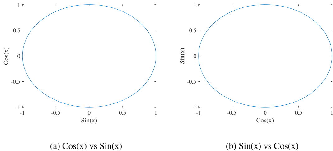
Figure 3.2: Phase Space
