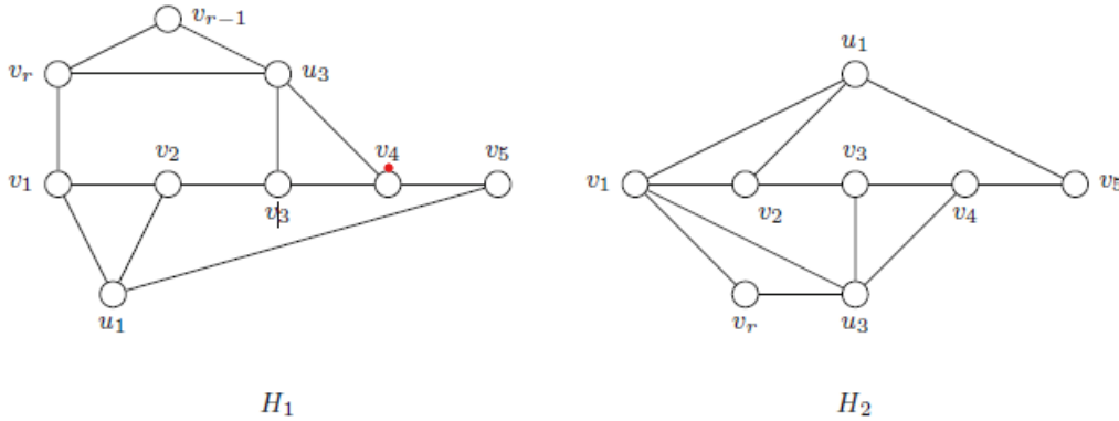
Fig. 1 The graphs H_1 and H_2
