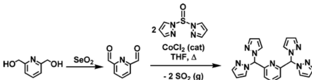
Scheme 1. Preparation of the pz 4 lut Ligand
