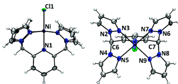
Figure 2. Two ORTEP (50% probability ellipsoids) views of the [NiCl(\mathbf{pz_4lut})]^+ cation.
