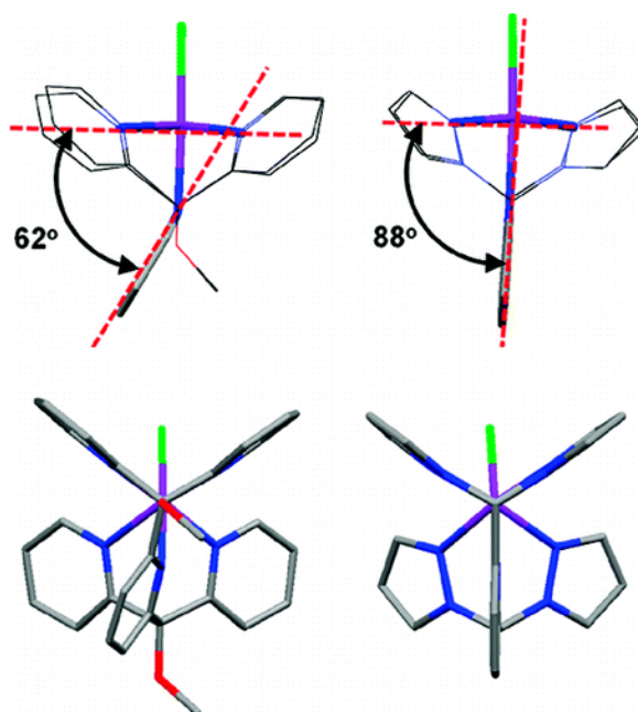
Figure 3. Comparison of the structures of related [NiCl(L)]^+ cations ( L = PY5 , left; L = \mathbf{pz_4lut} , right). H atoms are omitted. Top: views orthogonal to the axial pyridyl. Bottom: views down C–O ( PY5 ) or C–H ( pz 4 lut ) bonds.
