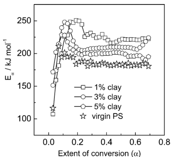
Figure 1 Dependence of the activation energy ( E_{\alpha} ) of degradation on the extent of conversion.
