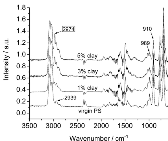
Figure 2 Gas phase IR spectra of degradation products.
