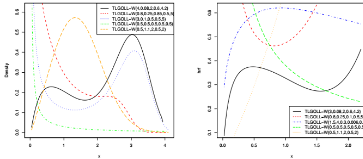
FIGURE 2. The pdf and hrf of the TLGOLL-W distribution for selected parameter values
