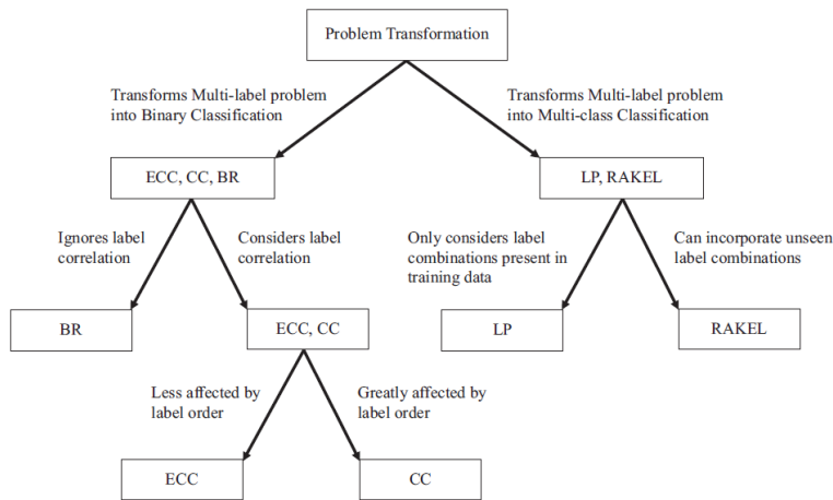
Figure 1 Relationships among problem transformation approaches.
