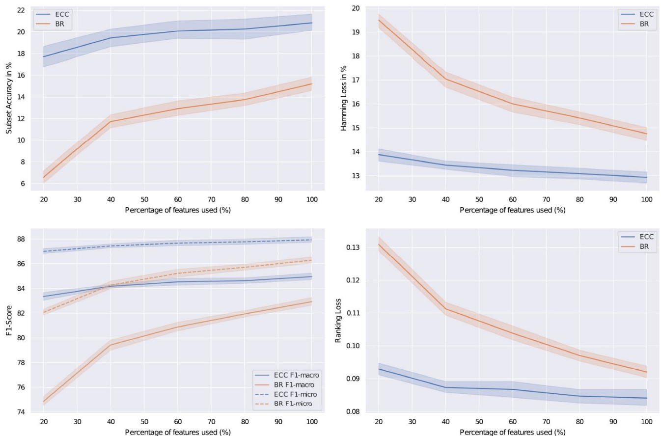
Figure 2 Performance of binary relevance (BR) and ensemble classifier chain (ECC) for the proposed metrics. Shaded regions denote the standard deviation of the bootstrap splits. For the metrics reported in the left-hand panels, higher values imply better performance. For the metrics reported in the right-hand panels, lower values imply better performance.
