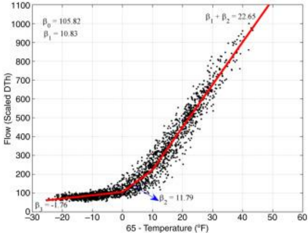
Fig. 1. The relationship between natural gas consumption and temperature for operating area 1. The red function captures the trend lines of the linear regression model for operating area 1, given by y_t = \beta_0 + \beta_1 \text{HDD}_{55} + \beta_2 \text{HDD}_{65} + \beta_3 \text{CDD}_{65} . (For the interpretation of the references to colour in this figure legend, the reader is referred to the web version of this article.)
