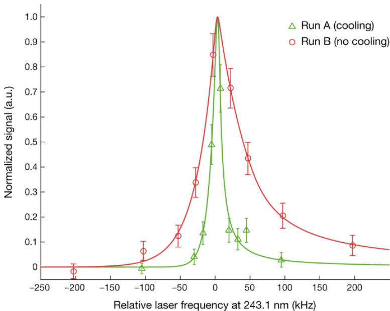
Fig. 5: Recorded spectra of the 1S–2S transition from runs A and B.
