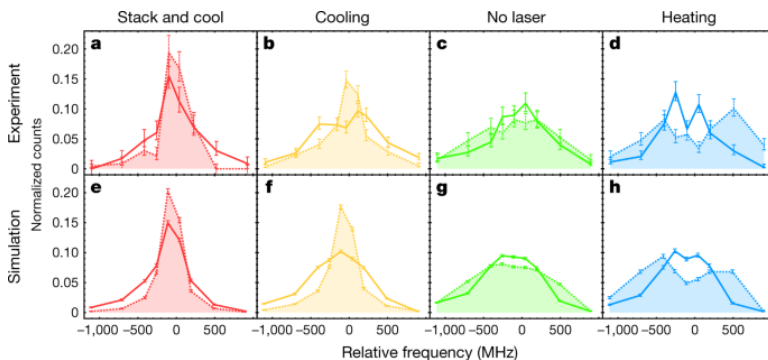
Fig. 4: Comparison of spectral lineshapes between transversely cold and hot anti-atoms within the same series in the cooling experiment.
