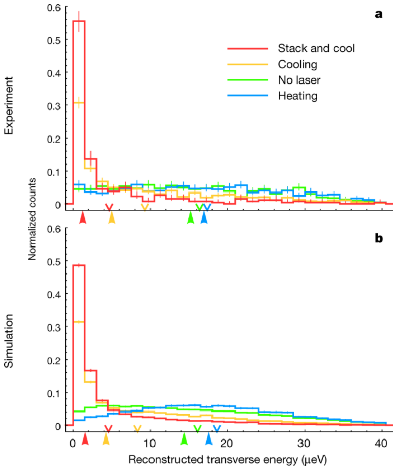
a , Distributions of the transverse kinetic energies reconstructed from the TOF of antihydrogen for different series. On the horizontal axis, the mean values of the reconstructed energies for each series are marked by downward-facing arrows, and the medians by upward-facing arrows. b , Corresponding simulations, where simulated events are analysed in the same way as above. The error bars represent 1 s.d. statistical uncertainties. See text and Methods.
