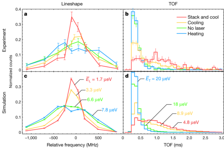
Fig. 2: Laser cooling of antihydrogen.
