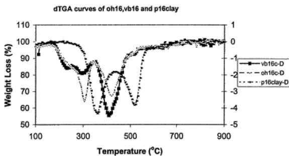
Figure 2 TGA curves for VB-16 and OH-16 clays under an inert atmosphere.
