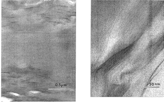
Figure 5 TEMs of the OH-16 nanocomposite at low (left) and higher (right) magnifications.
