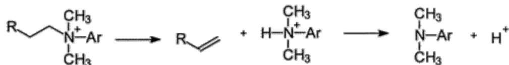
Scheme 1. Degradation of an “Onium” Salt To Give an Olefin, an Amine, and a Proton as the Counterion for the Clay
