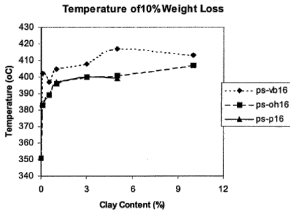
Figure 7 Temperature of 10% mass loss for nanocomposites as a function of the fraction of clay.
