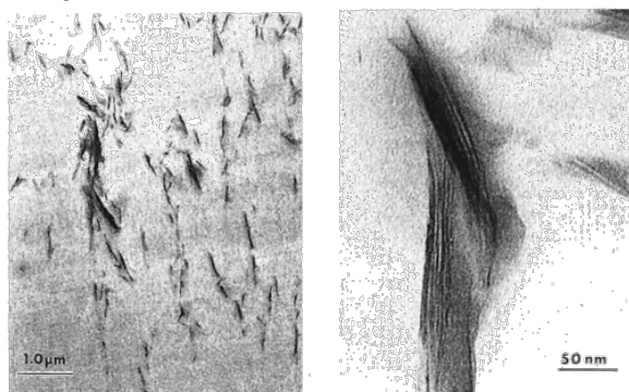
Figure 2 TEM images of the polystyrene nanocomposite of synthetic montmorillonite, SMM, derivatized with M2HTB.
