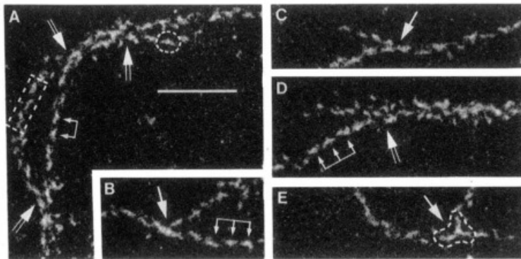
Fig 3.. STEM images of fibrils and fibril junctions. Fibrin was formed from fibrinogen fraction 1-2 solutions in 400 mmol/L NaCl, 10 mmol/L HEPES, 1 mmol/L CaCl 2 , pH 8.5 buffer (I = 0.4) (A through C), or in 400 mmol/L NaCl, 10 mmol/L HEPES, 5 mmol/L EDTA, pH 8.5 buffer (I = 0.4) (D and E). A “fiber” program (eg, rectangle in A) was used for determining fibril mass/length, a “circle” program (eg, circle in A) was used for estimating the mass of D · E · D complexes within fibrils, or a “user-defined boundary” program (eg, irregular enclosed shape in E) was used for measuring the mass at a junctional nidus. 20, 21 Bar = 100 nm.
