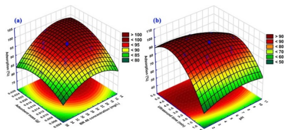
Fig. 3. The 3D response surfaces plot for the ultrasound-assisted adsorption of BR 46 dye.
