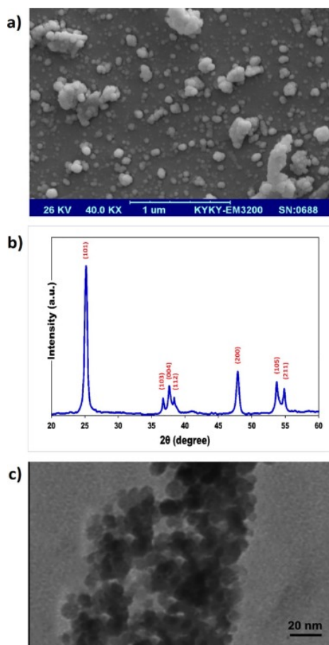
Fig. 1. FE-SEM (a), XRD (b), and TEM (c) of Ce-TiO 2 -NPs.
