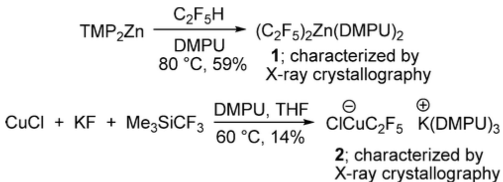
Scheme 3. Reaction Intermediate Synthesis
