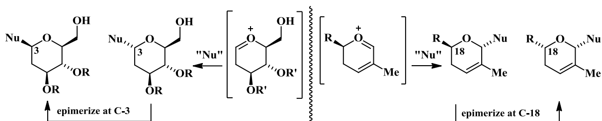
Figure 3. C-glycosylation and epimerization to cis -tetrahydro- and cis -dihydro-pyrans.
