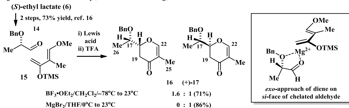
Scheme 4. Aldehyde-silyloxy diene cyclocondensation.
