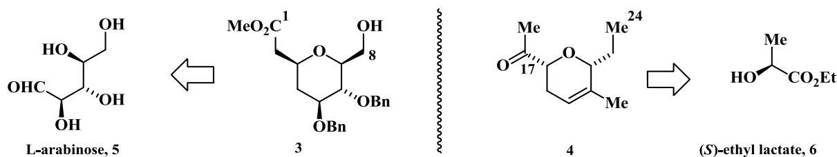
Figure 2. Retrosynthetic analysis of segments 3 and 4 into chiral pool precursors.
