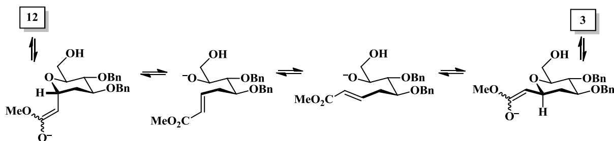
Scheme 3. Epimerization of trans - 12 to cis - 3 .
