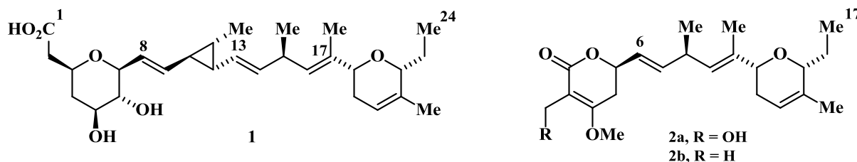
Figure 1. Structures of ambruticin ( 1 ) and the jerangolides ( 2a/b ).
