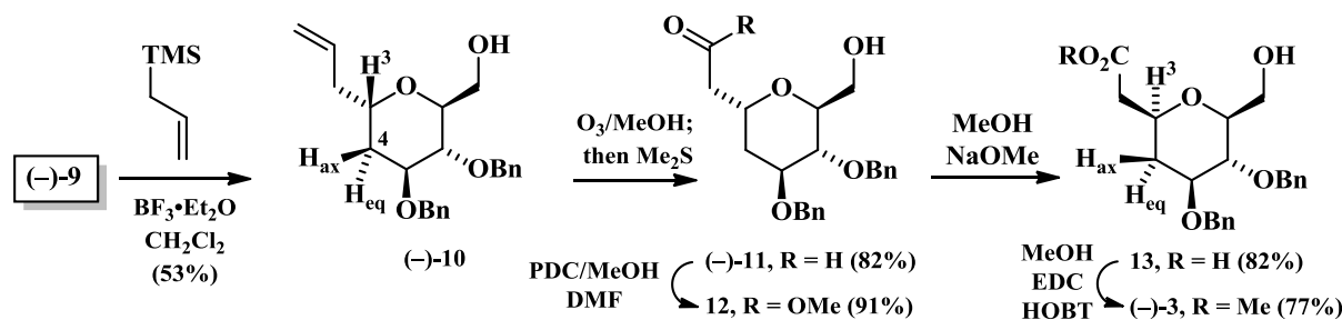
Scheme 2. Synthesis of the C1-C8 segment (-)- 3 .
