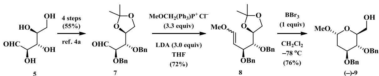
Scheme 1. Synthesis of the methyl 3,4-bis- O -benzyl-2-deoxy- L -glucoside (-)-9.
