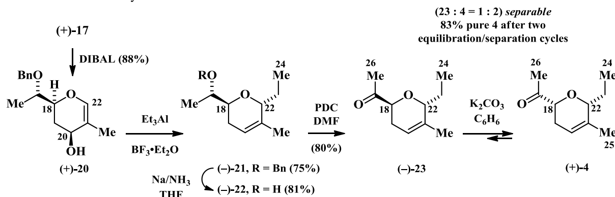
Scheme 5. Synthesis of dihydropyran segment 4 .
