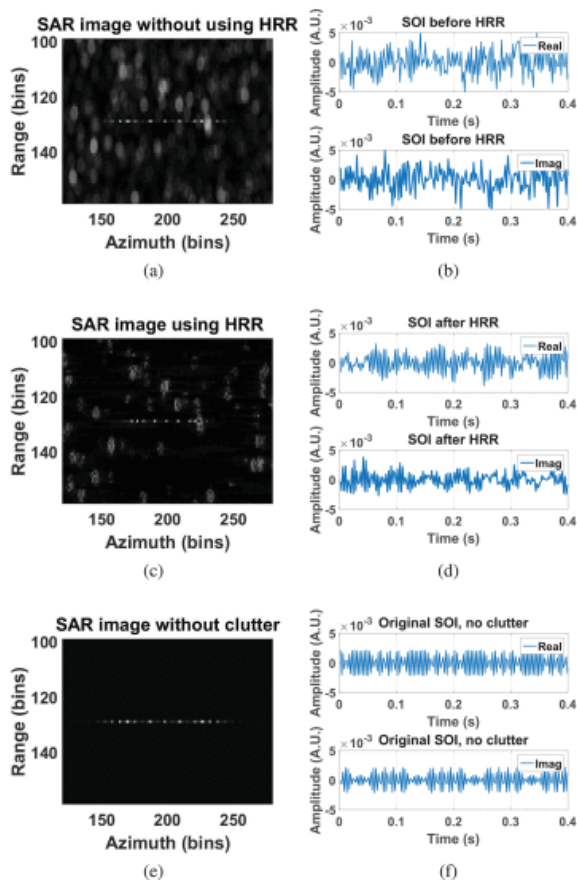
Fig. 2. Result of applying the HRR method on the range-compressed phase history of the simulated data. Magnitude of the SAR image (a) before applying the HRR method, (c) after applying the HRR method, and (e) vibrating target without clutter (reference). Slow-time SOI (b) before applying the HRR method, (d) after the applying HRR method, and (f) vibrating target without clutter (reference).
