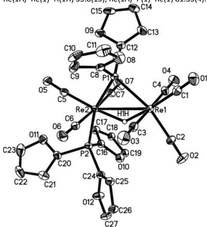
Fig. 4. Molecular structure of [\text{Re}_2(\text{CO})_7(\text{PFu}_3)(\mu\text{-PFu}_2)(\mu\text{-H})] (4) showing 50% probability thermal ellipsoids. Ring hydrogens are omitted for clarity. Selected bond distances ( \text{\AA} ) and angles( ^\circ ): \text{Re}(1)\text{-Re}(2) 3.1447(2), \text{Re}(1)\text{-}
