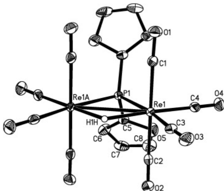
Fig. 3. Molecular structure of [\text{Re}_2(\text{CO})_8(\mu\text{-PFu}_2)(\mu\text{-H})] (3) showing 50% probability thermal ellipsoids. Ring hydrogens are omitted for clarity. Selected bond distances ( \text{\AA} ) and angles( ^\circ ): \text{Re}(1)\text{-Re}(1\text{A}) 3.1571(3), \text{Re}(1)\text{-P}(1) 2.4225(10), \text{P}(1)\text{-Re}(1\text{A}) 2.4225(10), \text{Re}(1)\text{-H}(1\text{H}) 1.95(4), \text{C}(4)\text{-Re}(1)\text{-C}(3) 93.54(16), \text{C}(2)\text{-Re}(1)\text{-C}(1) 178.16(15), \text{C}(3)\text{-Re}(1)\text{-P}(1) 169.20(12), \text{C}(4)\text{-Re}(1)\text{-Re}(1\text{A}) 146.54(12), \text{C}(3)\text{-Re}(1)\text{-Re}(1\text{A}) 119.87(12), \text{P}(1)\text{-Re}(1)\text{-Re}(1\text{A}) 49.34(2), \text{C}(4)\text{-Re}(1)\text{-H}(1\text{H}) 177.1(12), \text{C}(3)\text{-Re}(1)\text{-H}(1\text{H}) 84.1(15), \text{P}(1)\text{-Re}(1)\text{-H}(1\text{H}) 85.1(15), \text{Re}(1\text{A})\text{-Re}(1)\text{-H}(1\text{H}) 35.8(15), \text{Re}(1\text{A})\text{-P}(1)\text{-Re}(1) 81.33(4).
