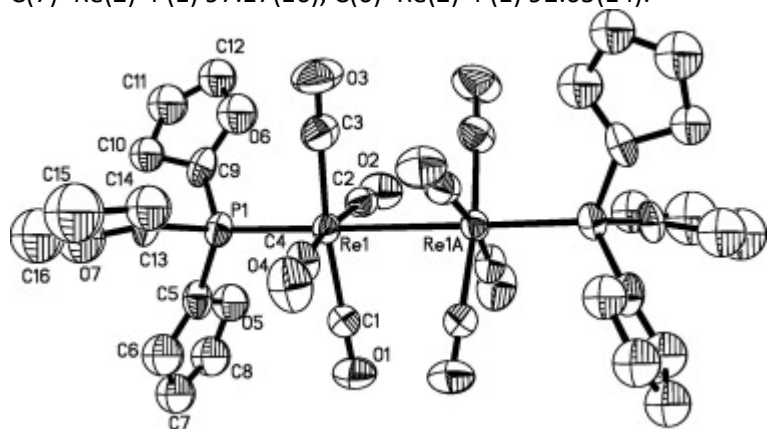
Fig. 2. Molecular structure of [\text{Re}_2(\text{CO})_8(\text{PFu}_3)_2] ( 2 ) showing 50% probability thermal ellipsoids. Ring hydrogens are omitted for clarity. Selected bond distances (Å) and angles(°): Re(1)–Re(1A) 3.0314(3), Re(1)–P(1) 2.3356(12), P(1)–Re(1)–Re(1A) 177.29(4), C(3)–Re(1)–P(1) 93.38(16), C(4)–Re(1)–P(1) 95.79(16), C(1)–Re(1)–P(1) 93.87(15), C(2)–Re(1)–P(1) 92.65(14), C(1)–Re(1)–C(3) 172.7(2), C(2)–Re(1)–C(4) 171.2(2).
