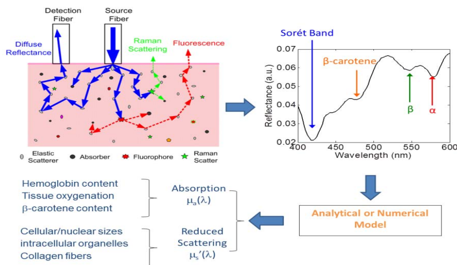
Figure 8: Illustration of the principle of diffuse reflectance spectroscopy with a fiber optic probe and the spectrum analysis procedures.
