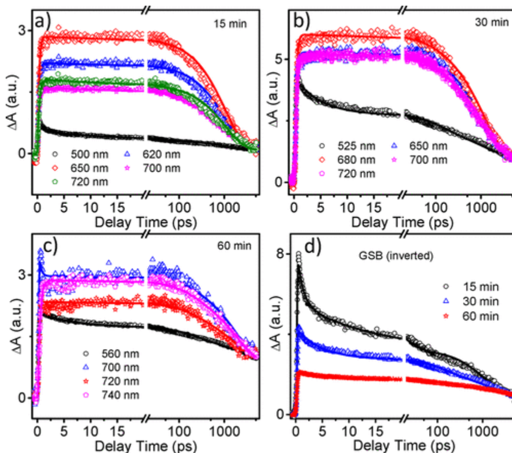
Figure 4. Comparison of OTA kinetic traces of CIS NPs at various probe wavelengths for samples with 15 min (a), 30 min (b), and 60 min (c) nucleation time following 480 nm excitation. (d) The comparison of ground-state bleach recovery kinetics (inverted) for 15, 30, and 60 min samples. These kinetic traces are normalized at 5 ns for better comparison.
