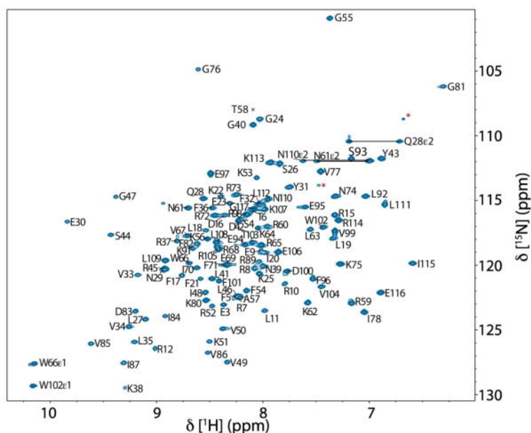
Fig. 1 900\text{ MHz } (^1\text{H}, ^{15}\text{N}) HSQC spectrum of 400\ \mu\text{M} T. maritima RNase P protein in 20\text{ mM} sodium phosphate (pH 6.0), 80\text{ mM} NaCl, 50\ \mu\text{M} DSS, 8\text{ mM} sodium sulfate, and 5\% \text{D}_2\text{O} at 318\text{ K} . Assigned residues are indicated using single letter codes . Side-chain \text{NH}_2 resonances of asparagine and glutamine are connected by horizontal lines . Signals labeled by red asterisks likely derive from arginine \epsilon\text{NH} resonances while those non-labeled are likely from minor population of the structural conformations in the sample. The assigned resonances with only a black cross indicate the position of the residue below the spectrum's intensity levels. Numbering of T. maritima RNase P protein corresponds to the gene sequence RNPA_THEMEA (UniProtKB - Q9X1H4).
