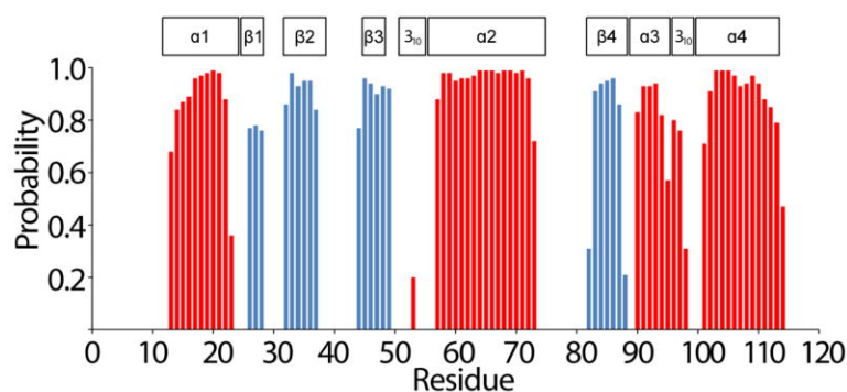
Fig. 2 TALOS-N prediction of secondary structure elements of T. maritima RNase P protein derived from H^N , N , H^\alpha , C^\alpha , C^\beta and C' chemical shifts. The secondary structure probability is reflected by the height of the bars (blue \beta -strand, red \alpha -helices). For comparison, the positions of secondary structure elements according to the crystal structure (PDB entry 1ZN0) are indicated above the amino acid residues.
