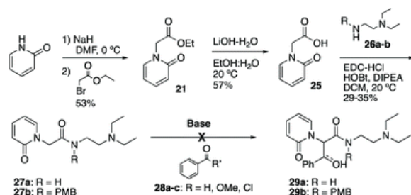
Scheme 6 C2–C3 coupling attempts on amide 26a–b .
