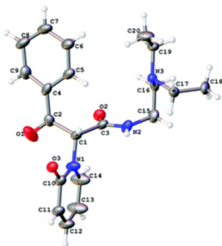
Fig. 3 X-ray structure of amide 61 .
