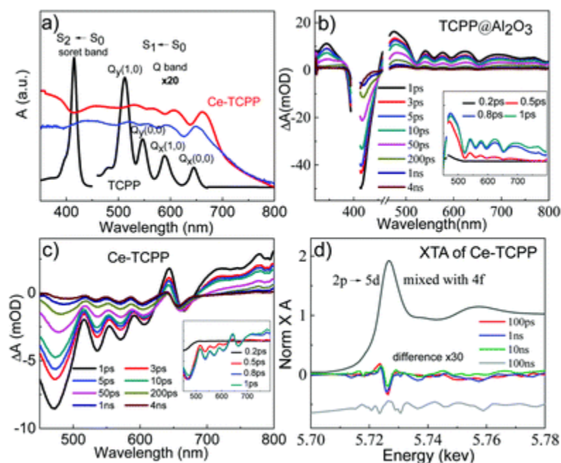
Fig. 3 (a) UV-visible absorption spectrum of TCPP in methanol and the diffuse reflectance spectrum of TCPP in the solid state (blue) and Ce–TCPP (red). OTA spectra of TCPP/ \text{Al}_2\text{O}_3 (b) and Ce–TCPP (c) following 400 nm excitation. The insets show the early time OTA spectra. (d) XANES spectrum of Ce–TCPP MOFs at the Ce L_3 -edge (black plot) and the difference XANES spectra at 100 ps (red), 1 ns (blue), 10 ns (green), and 100 ns (gray) obtained by subtracting the laser-off spectrum from the laser-on spectrum. The difference spectrum at 100 ns delay is shifted manually to provide an offset for a clearer view.
