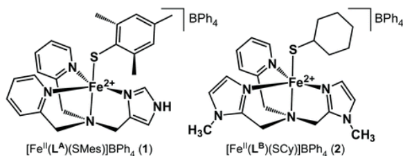
Scheme 2 Structures of complexes 1 and 2 .
