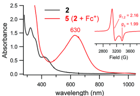
Fig. 2 UV-vis spectra of the oxidation of complex 2 (black line) to 5 (red line) via addition of one equivalent of [\text{Fc}]\text{PF}_6 . The reaction occurred in \text{CH}_3\text{CN} at -40\text{ }^{\circ}\text{C} . The initial concentration of 2 was 0.90 mM. Inset: X-band EPR spectrum of 5 measured at 10 K in frozen \text{CH}_3\text{CN} . Data were collected at a frequency of 9.39 GHz and power of 2.0 mW.
