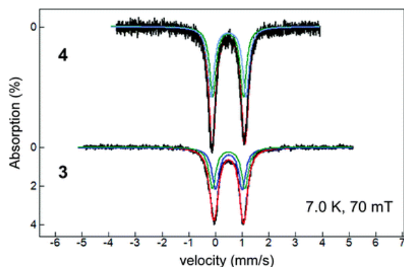
Fig. 3 Mössbauer spectra of complexes 3 and 4 measured at 7.0 \text{ K} and 70 \text{ mT} , prepared as described in the text. The hatch marks are the experimental data, and the colored lines are spectral fits generated with the parameters in Table 1. For clarity, both spectra were prepared by removing the unreacted Fe(II) species from the raw data.
