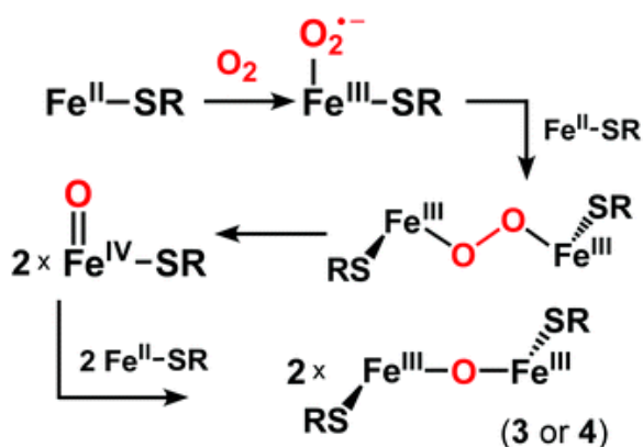
Scheme 3 Proposed mechanism for formation of intermediates 3 and 4 .
