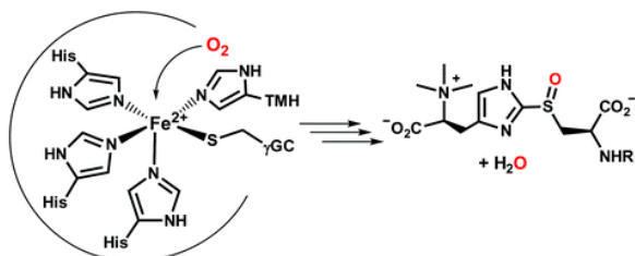
Scheme 1 Substrate-bound active site and product of EgtB.
