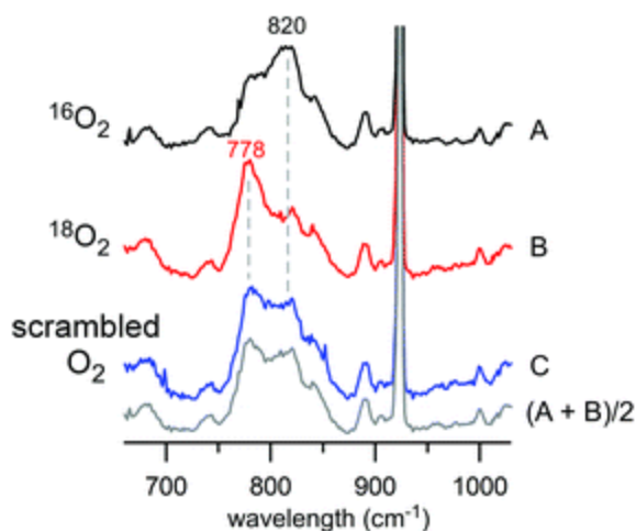
Fig. 6 Resonance Raman spectra of 4 in frozen CH 3 CN collected using 501.7 nm excitation (24–30 mW at sample). The samples were prepared by treating 10 mM solutions of 2 with 16 O 2 (A, black line), 18 O 2 (B, red line), or scrambled O 2 (C, blue line). The bottom spectrum (gray line), generated by digital addition, is half the sum of spectra A and B. Solvent-derived peaks were used to normalize spectral intensities.
