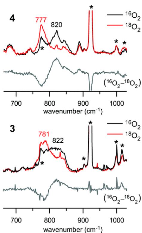
Fig. 5 Resonance Raman spectra of 4 (top) and 3 (bottom) in frozen CH 3 CN (77 K). Samples were prepared using either 16 O 2 (black lines) or 18 O 2 (red lines). Derivative-shaped features in the 16 O 2 – 18 O 2 difference spectra (gray lines) are due to isotopically-active peaks. All spectra were measured using 501.7 nm laser excitation at a power of 20–30 mW at the sample. The solvent-derived features marked with an asterisk (*) were used to normalize spectral intensities.
