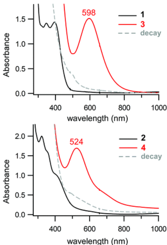
Fig. 1 UV-vis absorption spectra of the reaction of 1 (top) and 2 (bottom) with O 2 in CH 3 CN at -40 °C. Spectra of the Fe(II) precursors ( 1 and 2 ) and O 2 -generated intermediates ( 3 and 4 ) are shown as black and red lines,
