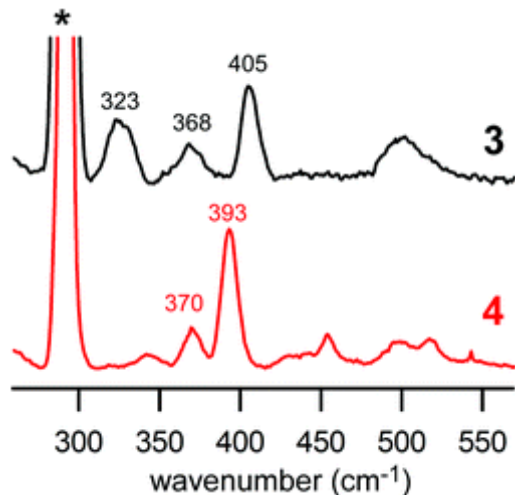
Fig. 7 Resonance Raman spectra of 3 and 4 in frozen CD 2 Cl 2 (77 K). Spectra were collected with laser excitation of 514.5 nm ( 3 ) and 501.7 nm ( 4 ). Samples were prepared by addition of O 2 to solutions of the precursor complexes. The solvent-derived peak marked with an asterisk (*) was used to normalize spectral intensities.
