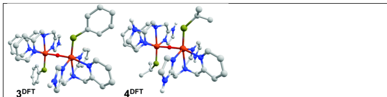
Fig. 8 DFT geometry-optimized models of intermediates 3 and 4 . Most hydrogen atoms are omitted for the sake of clarity. The thiolate ligands have been modified as described in Computational Methods. Atomic colors: C, gray; N, blue; O, red; S, yellow; Fe, orange.
