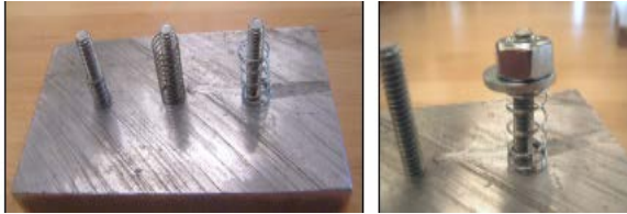
Figure 10. Fixture for testing mechanical wire springs.
