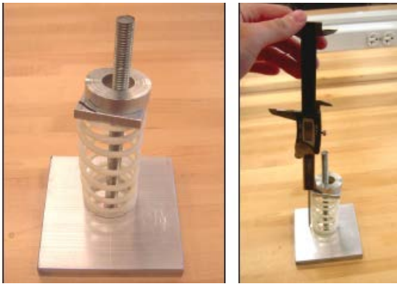
Figure 9. Testing 3D printed springs.
