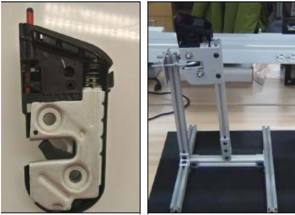
Figure 2. STRATTEC Seatback latch (left) and test fixture (right).
