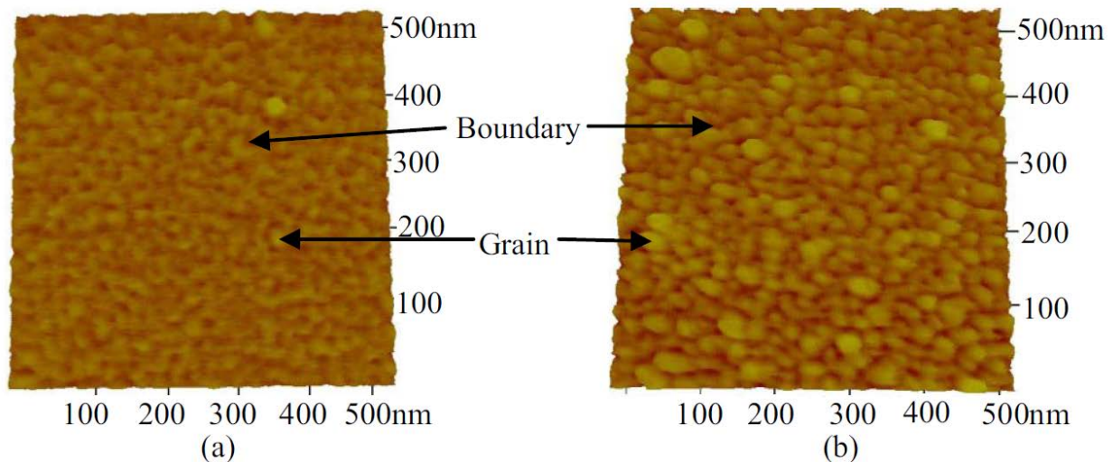
Fig. 1. AFM image of as-deposited 100 Å of (a) evaporated Ni and (b) sputtered Ni.
