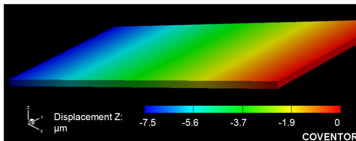
Fig. 3. CoventorWare finite element model of cantilever deflection for a static 1 \text{ kPa} applied load.
