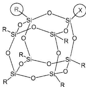
Figure 1 Generalized structure of a POSS material
