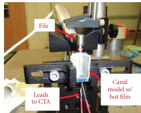
FIGURE 2: Hot-film experimental model.
