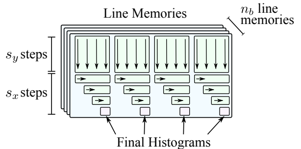
Figure 4: Parallel computation of the histograms.
