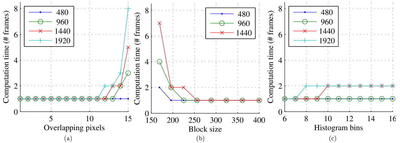
Figure 7: Computation time of the HOG-based tracker as a function of (a) the number of overlapping pixels, (b) the block size, and (c) the number of bins.
