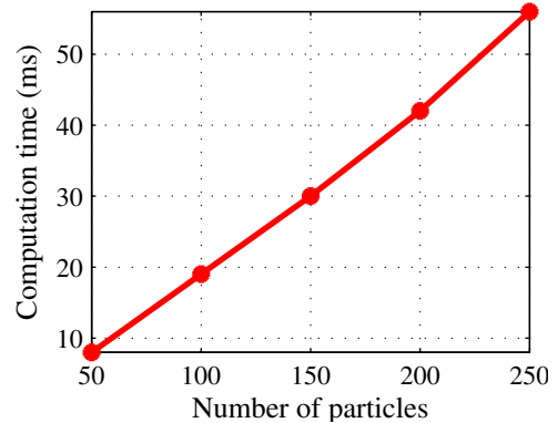
Figure 11: Resampling computation times in a low-power general-purpose processor.
